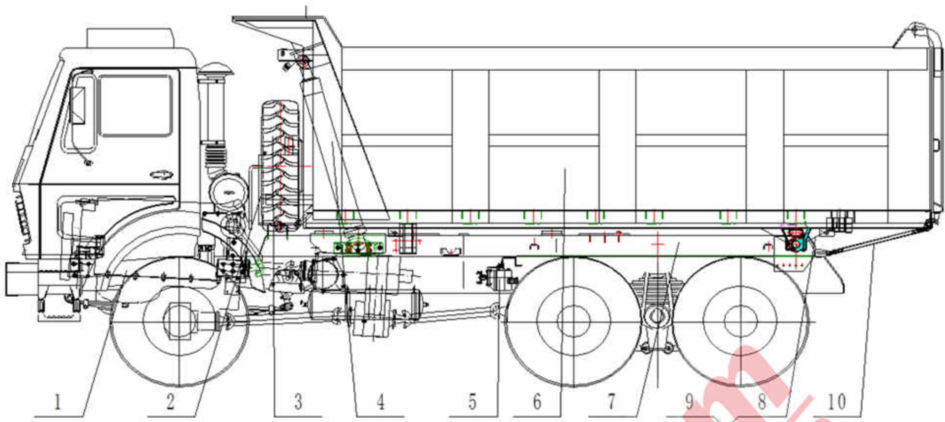
Sample Drawing for Dump Truck (6x4 model)
